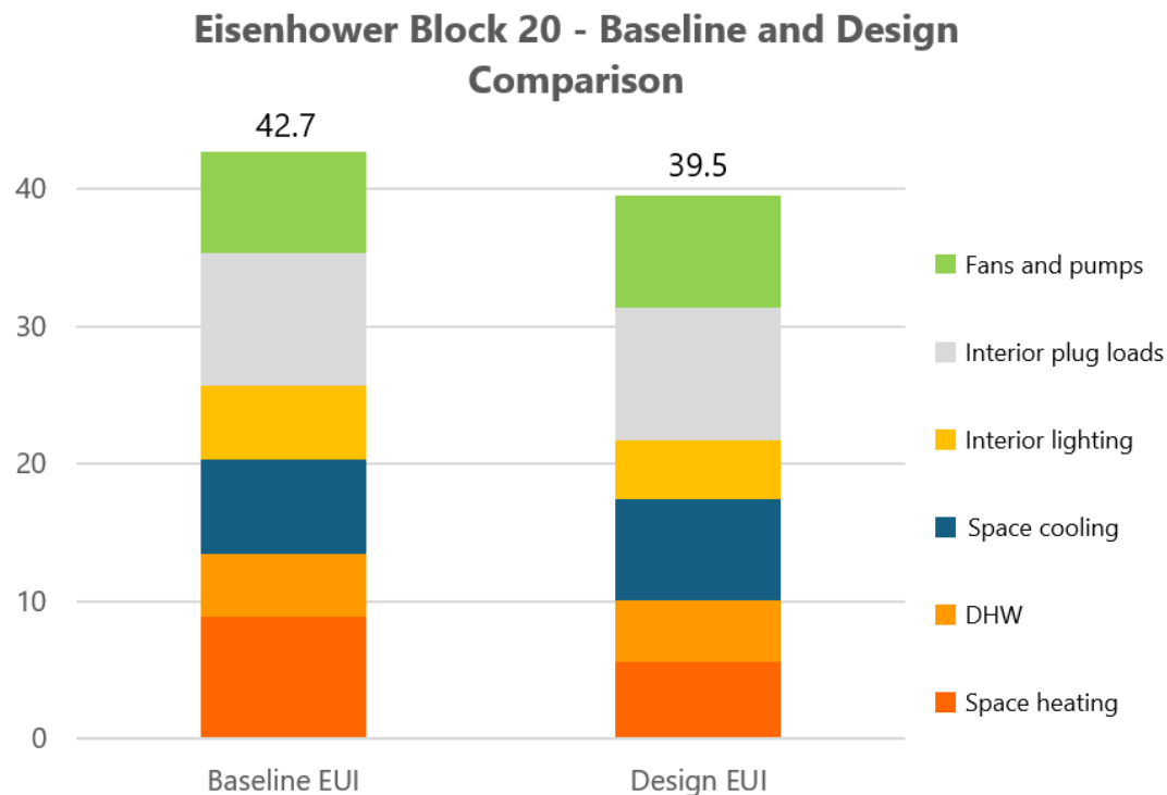
Figure 2: Baseline and Design EUI Comparison
