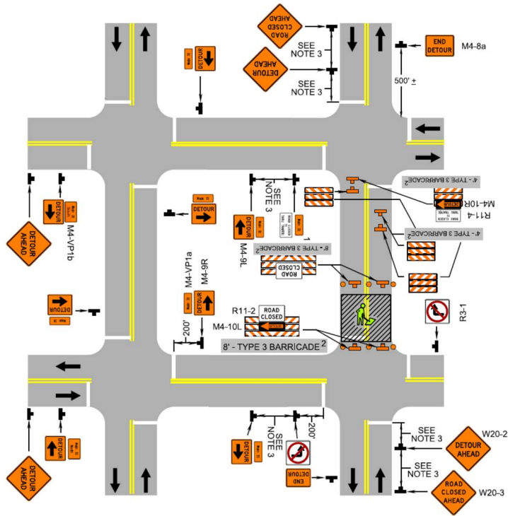
Street Closure Operation with Detour (Figure TTC-34.2)
