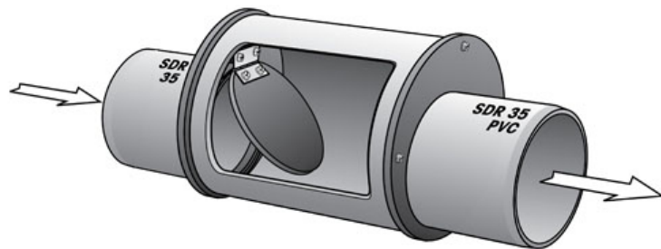
Check valves (one-way flow gates) within the storm sewer to prevent backflow
