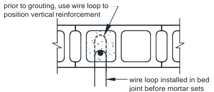
FIGURE 5: VERTICAL REINFORCEMENT TIE-HOLD DETAIL
