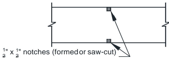
FIGURE 10: CONCRETE CONTROL JOINT DETAIL
