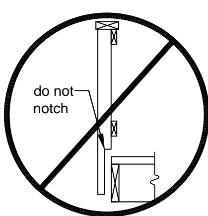
FIGURE 36: POST NOTCHES PROHIBITED
