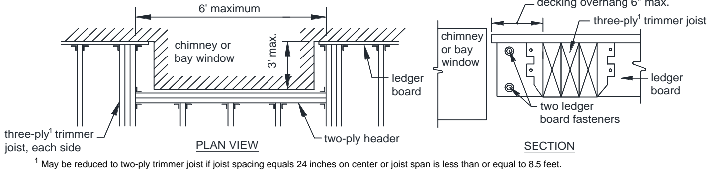
FIGURE 10: FRAMING AT CHIMNEY OR BAY WINDOW
