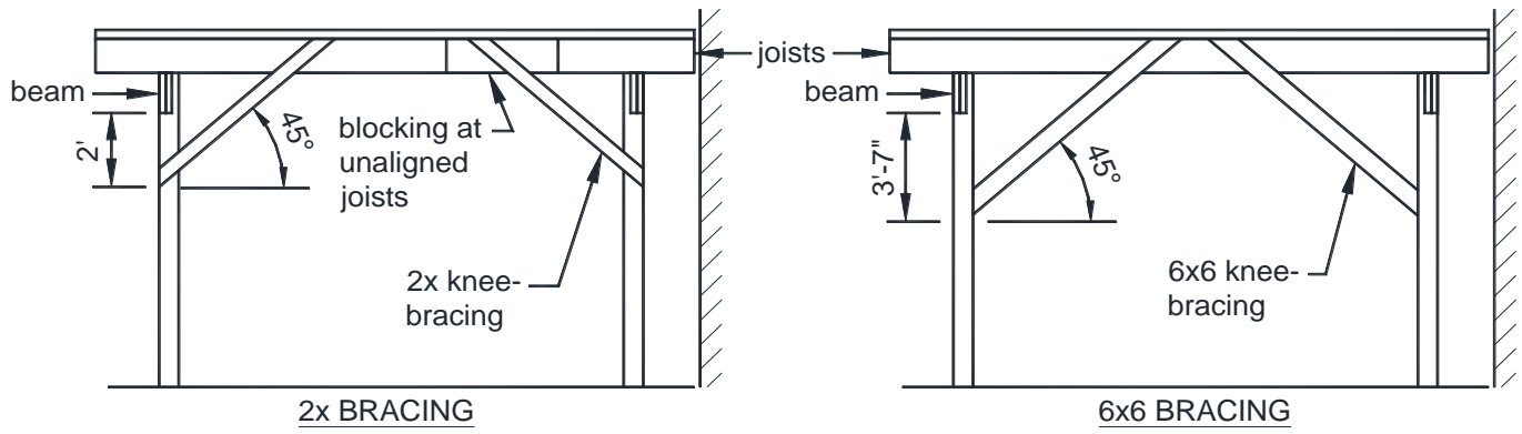
FIGURE 31: METHOD 3 - KNEE-BRACING AT JOIST-POST LOCATIONS
