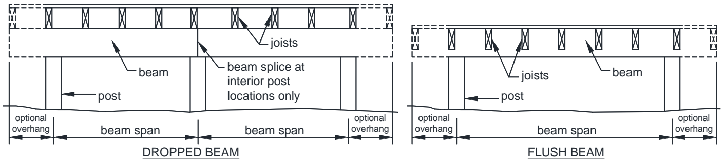
FIGURE 13: BEAM TYPES
