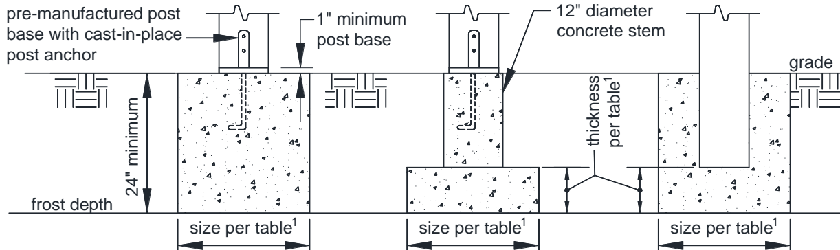
FIGURE 17: FOOTINGS
