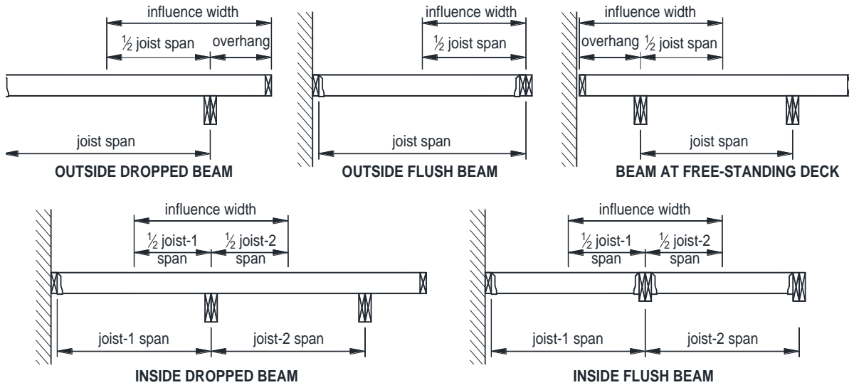
FIGURE 13: BEAM TYPES
