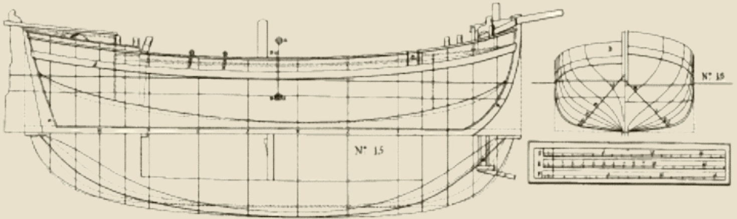
Chapman's Lighter No. 15 (Adapted from Chapman 1765, Pl. XXX, no. 15)
